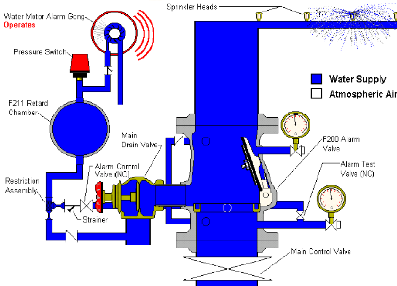
(6) Water Motor Alarm Gong Operates
